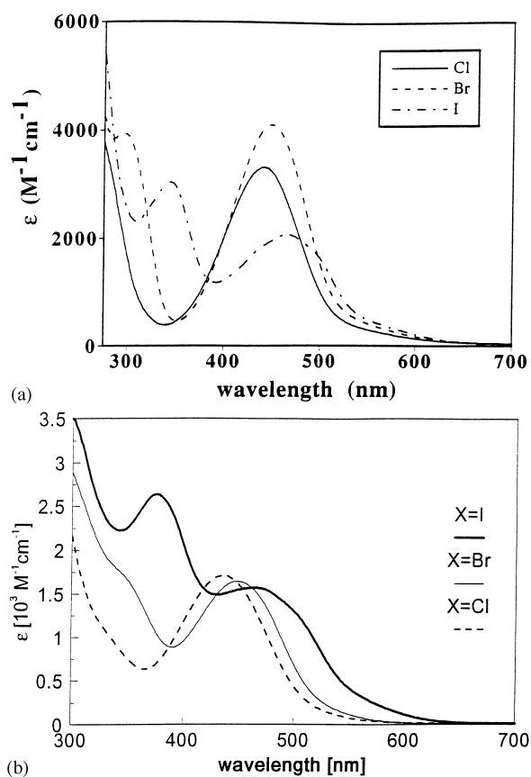
Fig. 9. (a) Electronic absorption spectra of \text{Re}(\text{X})(\text{CO})_3(i\text{Pr-DAB}) ; \text{X} = \text{Cl} , Br, I; measured in THF at r.t. [112]; (b) electronic absorption spectra of \text{Ru}(\text{X})(\text{Me})(\text{CO})_2(i\text{Pr-DAB}) ; \text{X} = \text{Cl} , Br, I; measured in THF at r.t. [76].
