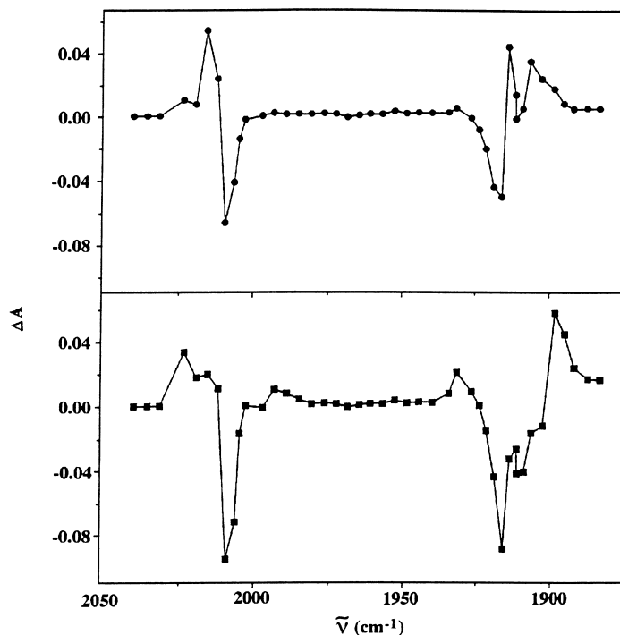
Fig. 11. Time-resolved IR spectra of Re(Bz)(CO) 3 ( i Pr-DAB) measured in n -heptane [57]. Negative bands correspond to bleached ground state while the positive ones belong to the photoproduct transients. Top: spectrum obtained at 100 ns after excitation corresponds to the \sigma\pi^* state. Bottom: spectrum obtained at 3.5 \mu\text{s} corresponds to the solvated Re(CO) 3 ( i Pr-DAB) • radical.
